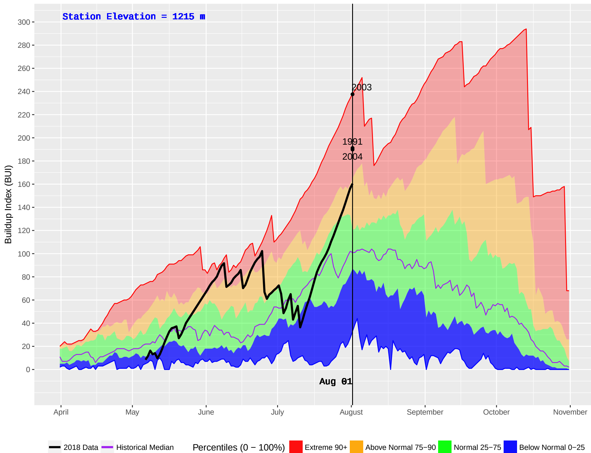
ALLISON PASS (317) : Historical (1987–2016) and Current (2018) Daily Buildup Index (BUI)
